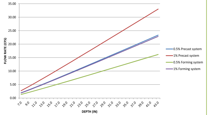
12" I.D. DURA TRENCH
