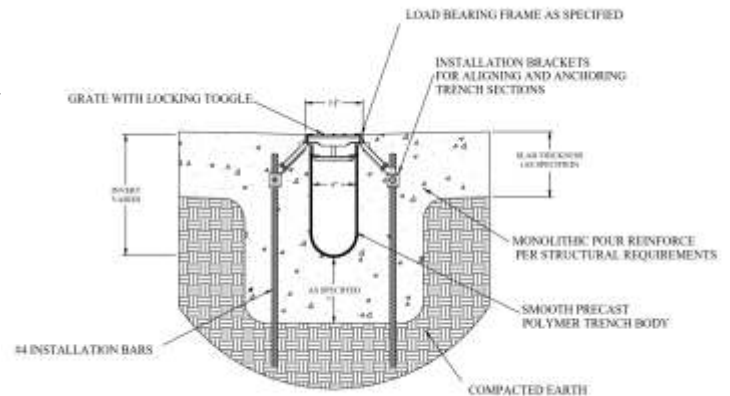
TYPICAL DTPF4 TRENCH SECTION
