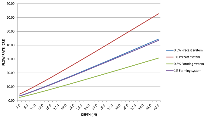
18" I.D. DURA TRENCH
