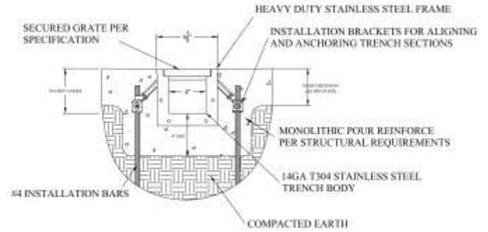
TYPICAL DTSS4 TRENCH SECTION
