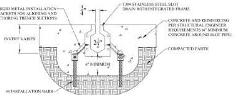
TYPICAL DTSS2 TRENCH SECTION
