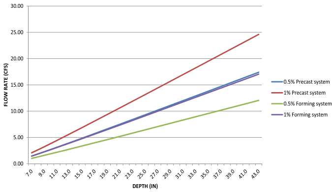
10" I.D. DURA TRENCH
