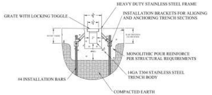
TYPICAL DTSS2 TRENCH SECTION
