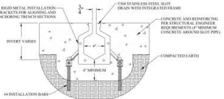
TYPICAL DTSSP4 TRENCH SECTION
