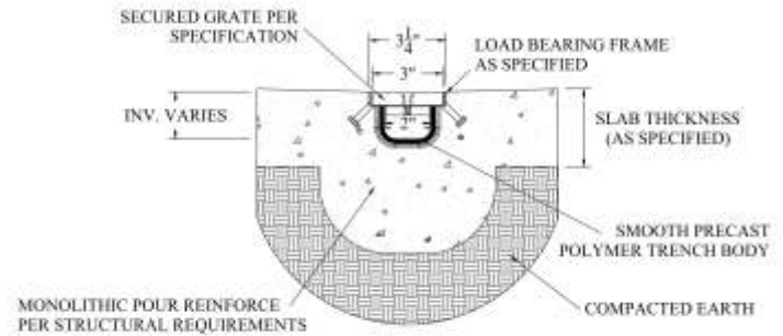
TYPICAL DTPF2 TRENCH SECTION
